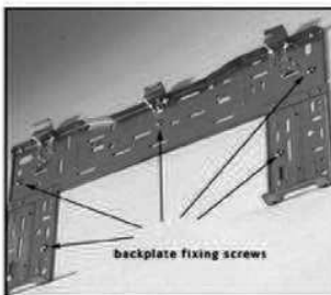
8. Fix the backplate to the wall.
