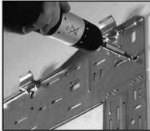
5. Screw the backplate to the wall using 1.5 inch number 10 screws.
